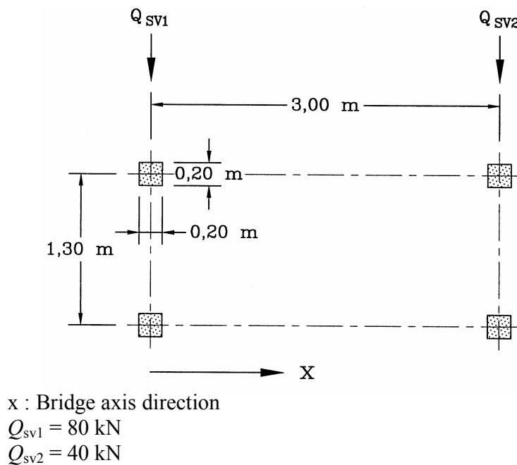
Figure 35. Service or Accidental vehicle
