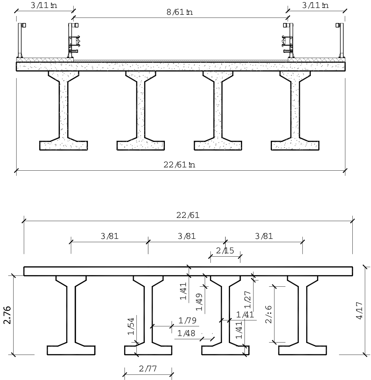
Figure 2: characteristics of the bridge transverse section (unit: m).
