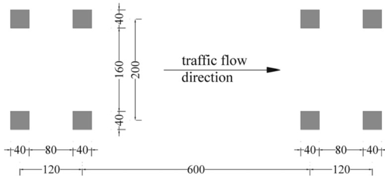
Fig. 25.b. Fatigue load model n. 1 for local verifications
