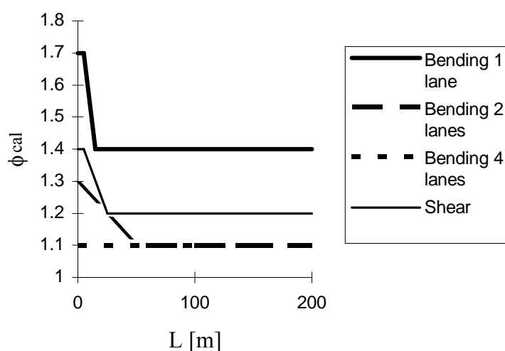
Fig. 10. Calibration value of the impact factors \varphi_{\text{cal}} (EC1).
