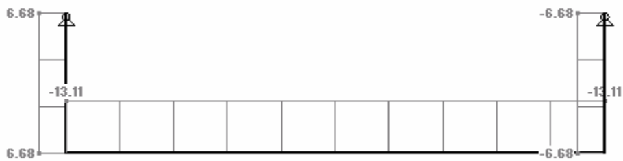
Figure 23. Distribution of axial forces [kN] in the frame structure
