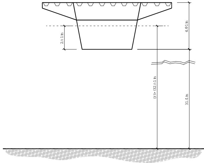
Figure 5: definition of z_e , the bridge's equivalent height, with the aim of evaluating wind actions.
