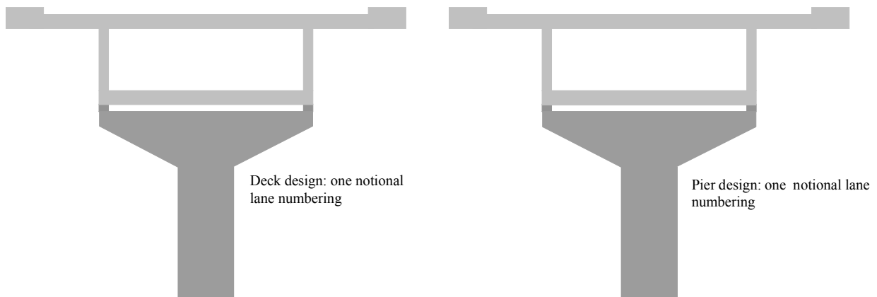
Fig. 12. Lane numbering – carriageway consisting of two separate parts on the same deck
