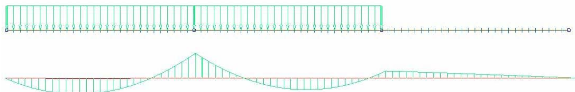
Figure 15: arrangement of the distributed traffic load to determine the maximum negative bending moment in absolute value on the first intermediate support.
