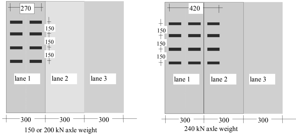
Fig. 18. Arrangement of special vehicle on the carriageway
