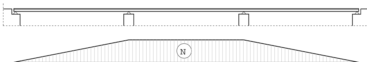
Figure 16: diagram of the bending moment for a linear temperature gradient through the section's thickness.
