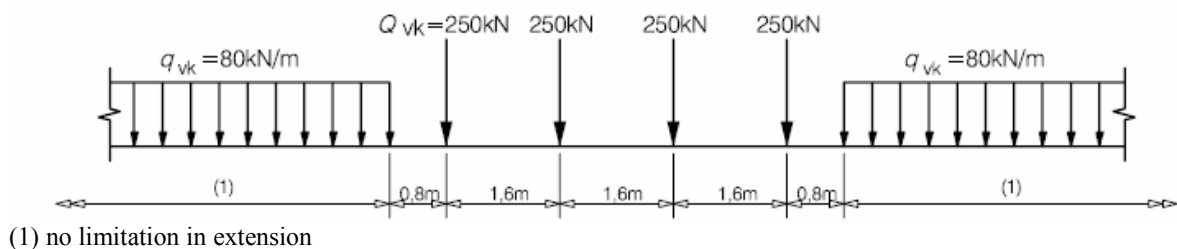
Figure 37. Load Model 71
