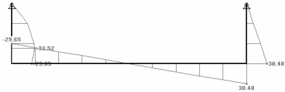
Figure 22. Moment distribution [kNm] at the frame structure
