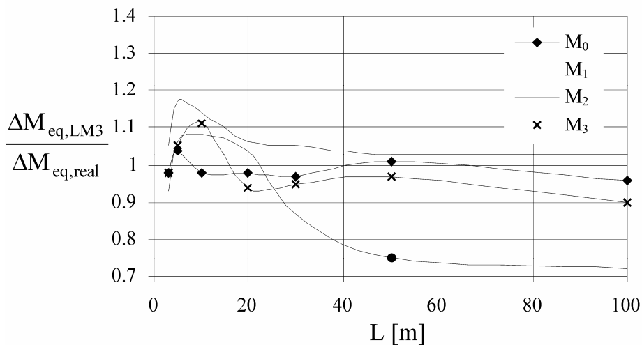
Figure 31. Accuracy of fatigue load model n. 3 – m=5
