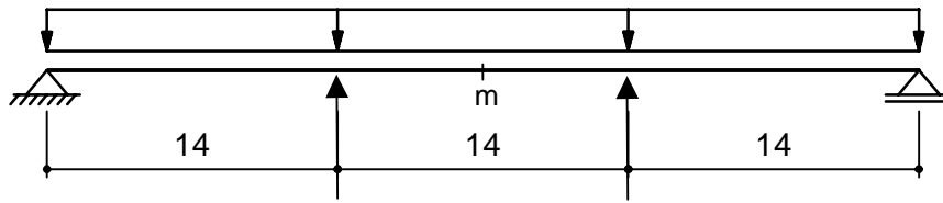
Figure 7. Characteristic value and combination value of the load on the footway
