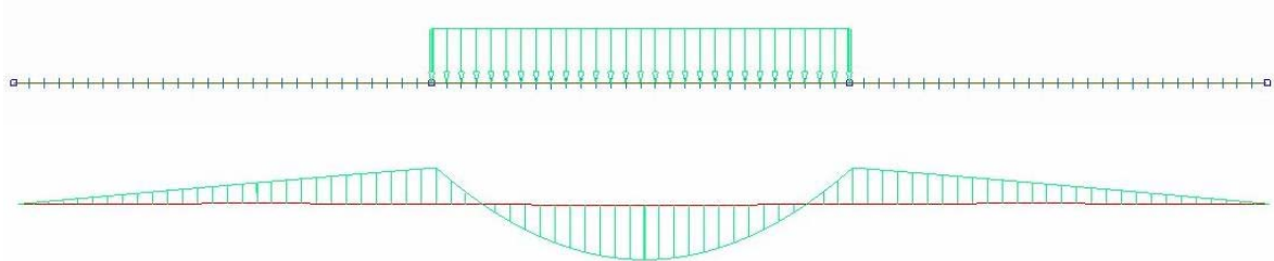
Figure 13: arrangement of the distributed traffic load maximizing the positive moment in the central span.
